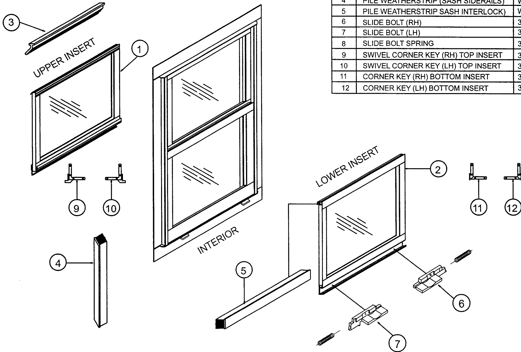
SERIES #17 HORIZONTAL/SERIES #18 VERTICAL SELF-STORING STORM WINDOW REPLACEMENT PARTS
